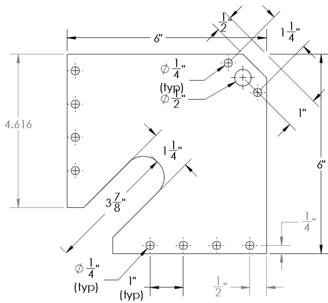
Base Plate 1/4" plate
